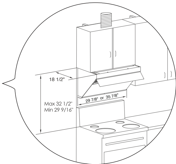
Under-Cabinet Installation
