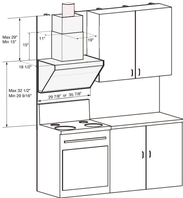
Wall-Mount Installation
