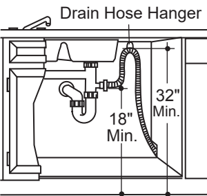
Waste Tee Installation
