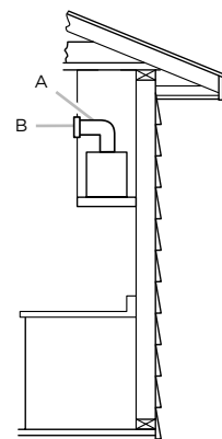
A. 6" (15.2 cm) vent through the cabinet B. B. Round recirculating grid
